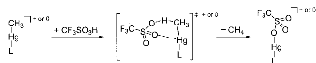
Scheme 4. Pathway of the reaction between [\text{MeHgL}]^+ \text{ or } 0 and trifluoromethanesulfonic acid ( \text{L} = \text{Cl}^- , \text{SEt}_2 , \text{MeSCH}_2\text{CH}_2\text{SMe} , or [9]\text{aneS}_3 )
