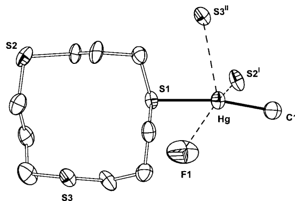
Figure 2. Ellipsoid plot (50% probability level) of the [\text{MeHg}(\text{12]aneS}_3)]^+ complex in crystals of 2 (hydrogen atoms are omitted); bond lengths [Å] and angles [°]: Hg–S1 2.441(4), Hg–C1 2.11(2), Hg \cdots S2 1 3.176(4), Hg \cdots S3 11 3.256(4), Hg \cdots F1 2.97(1); S1–Hg–C1 168.1(6); symmetry transformations: 1 : 0.5 + x , 0.5 – y , 0.5 + z ; 11 : 0.5 + x , 0.5 + y , z
