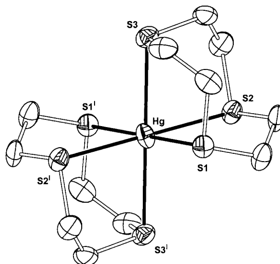
Figure 4. Ellipsoid plot (50% probability level) of the [\text{Hg}([9]\text{aneS}_3)_2]^{2+} complex in crystals of 4 (hydrogen atoms are omitted); bond lengths [Å] and angles [°]: \text{Hg-S1} 2.677(1), \text{Hg-S2} 2.660(1), \text{Hg-S3} 2.711(1); \text{S1-Hg-S2} 83.69(3), \text{S1-Hg-S3} 82.49(3), \text{S1-Hg-S1'} 180.0, \text{S1-Hg-S2'} 96.31(3), \text{S1-Hg-S3'} 97.51(3), \text{S2-Hg-S3} 83.14(3), \text{S2-Hg-S2'} 180.0, \text{S2-Hg-S3'} 96.86(3), \text{S3-Hg-S3'} 180.0; symmetry transformation: 1: -x, 1 - y, -z
