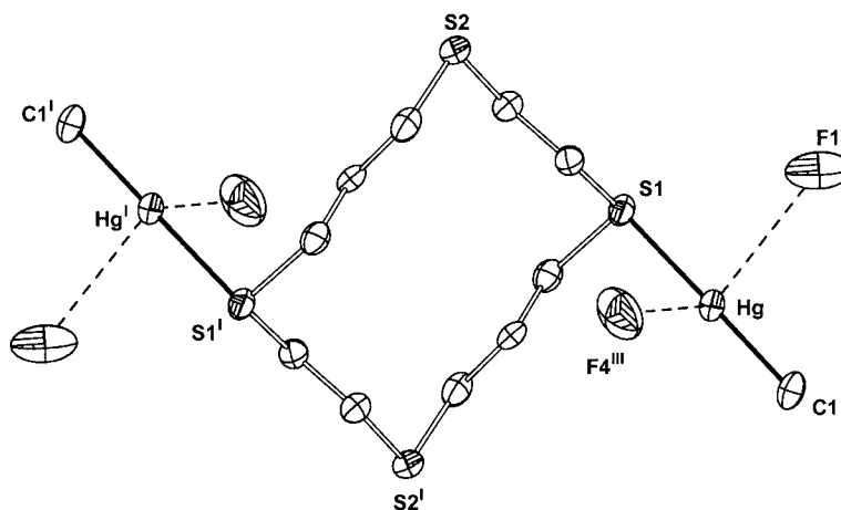
Figure 3. Ellipsoid plot (50% probability level) of the [(\text{MeHg})_2(\text{14]aneS}_4)]^{2+} complex in crystals of 3 (hydrogen atoms are omitted); bond lengths [Å] and angles [°]: Hg–S1 2.425(2), Hg–C1 2.068(7), Hg \cdots F1 11 2.947(5), Hg \cdots F4 111 2.946(5); S1–Hg–C1 174.7(2); symmetry transformations: 1 : – x , 2 – y , 2 – z ; 11 : –0.5 + x , 1.5 – y , –0.5 + z ; 111 : 0.5 – x , 0.5 + y , 1.5 – z
