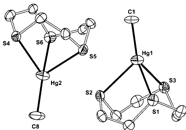
Figure 1. Ellipsoid plot (50% probability level) of the two symmetry-independent [\text{MeHg}(\text{9]aneS}_3)]^+ complexes in 1 showing their mutual orientation in the crystal (hydrogen atoms are omitted); bond lengths [Å] and angles [°]: Hg1–S1 2.611(2), Hg1–S2 2.768(2), Hg1–S3 2.760(2), Hg1–C1 2.080(8), Hg2–S4 2.720(2), Hg2–S5 2.732(2), Hg2–S6 2.677(2), Hg2–C8 2.075(8); S1–Hg1–S2 81.1(1), S1–Hg1–S3 79.6(1), S2–Hg1–S3 79.0(1), S1–Hg1–C1 142.7(4), S2–Hg1–C1 124.9(3), S3–Hg1–C1 127.3(4), S4–Hg2–S5 79.9(1), S4–Hg2–S6 80.4(1), S5–Hg2–S6 80.4(1), S4–Hg2–C8 132.2(3), S5–Hg2–C8 126.6(4), S6–Hg2–C8 136.4(4)
