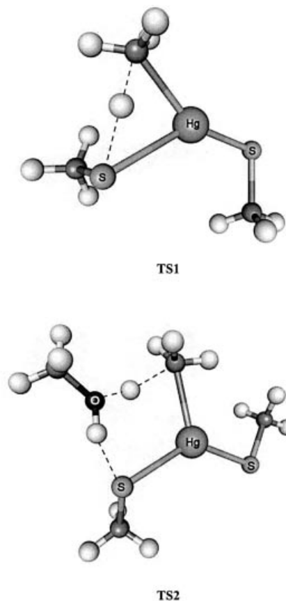
Figure 5. MP2/I-calculated transition states for the protonolytic Hg–C bond cleavage in \text{MeHg}(\text{SMe}) by methanethiol with (TS2), and without (TS1) assistance by methanol
