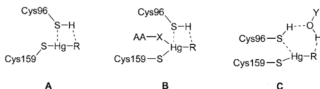
Scheme 3. Proposals for the key step of the reaction mechanism of organomercurial lyase; A: with only Cys96 and Cys159 being involved; B: with a further primary ligand \text{AA-X}^- , for example Tyr93 ( \text{X} = \text{O} ) or Cys117 ( \text{X} = \text{S} ); C: with participation of an additional amino acid (or water) \text{Y-OH} as a simultaneous proton donor and acceptor
